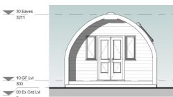
Front Elevation 1 : 50
