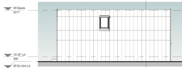
Side Elevation 1 1 : 50
